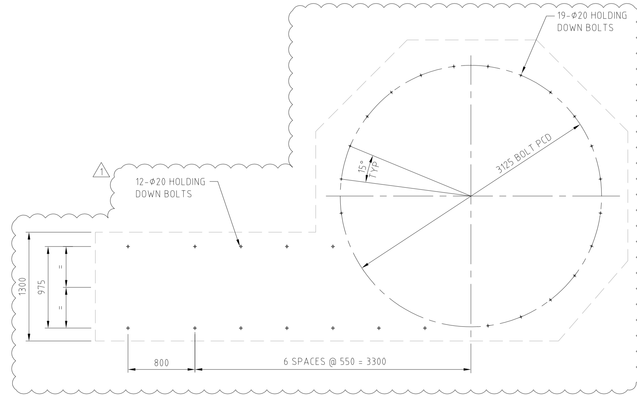
HOLDING DOWN BOLT SET OUT PLAN
